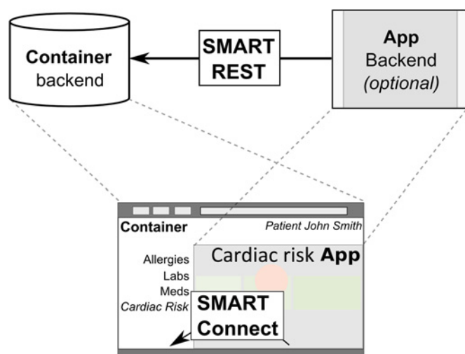
Figure 3 At the center, a web browser window presents two principal components: (1) a white border region belongs to the SMART container, displaying a list of available applications (apps) as well as patient context; (2) a larger gray block belongs to a single ‘Cardiac Risk’ app. As illustrated, the ‘Cardiac Risk’ app can request data from the container directly inside the browser via SMART Connect; an app with a back-end component may request data with a server-to-server call via SMART REST. In either case, the SMART-enabled electronic medical record or personally controlled health record responds with the same SMART RDF data payload.
